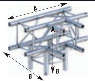
4-way T-piece System 29/4: A = 710 B = 500 mm System 39/4: A = 810 B = 600 mm
