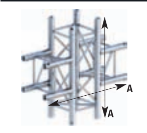
4-way cross System 29/4: A = 710 mm System 39/4: A = 810 mm
