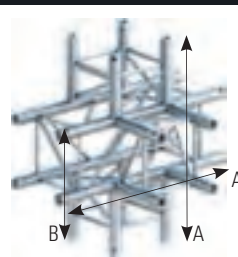
5-way cross System 29/4: A = 710 mm B = 500 mm System 39/4: A = 810 mm B = 600 mm
