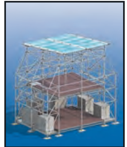
FOH-Tower 4 x 4 – 2 levels
