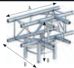
4-way T-piece System 29/4: A = 710 mm B = 500 mm System 39/4: A = 810 mm B = 600 mm
