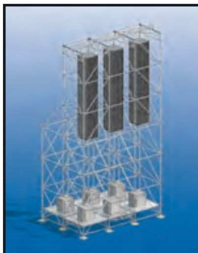
PA Wing 6 x 4
