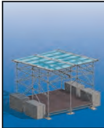
FOH-Tower 4 x 4 – 1 level
