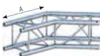
2-way corner 135° System 29/4: A = 500 mm System 39/4: A = 600 mm
