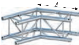
2-way corner 120° System 29/4: A = 500 mm System 39/4: A = 600 mm
